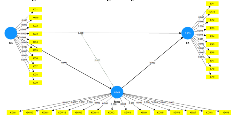
FIGURE 2. BOOTSTRAPPING ANALYSIS
